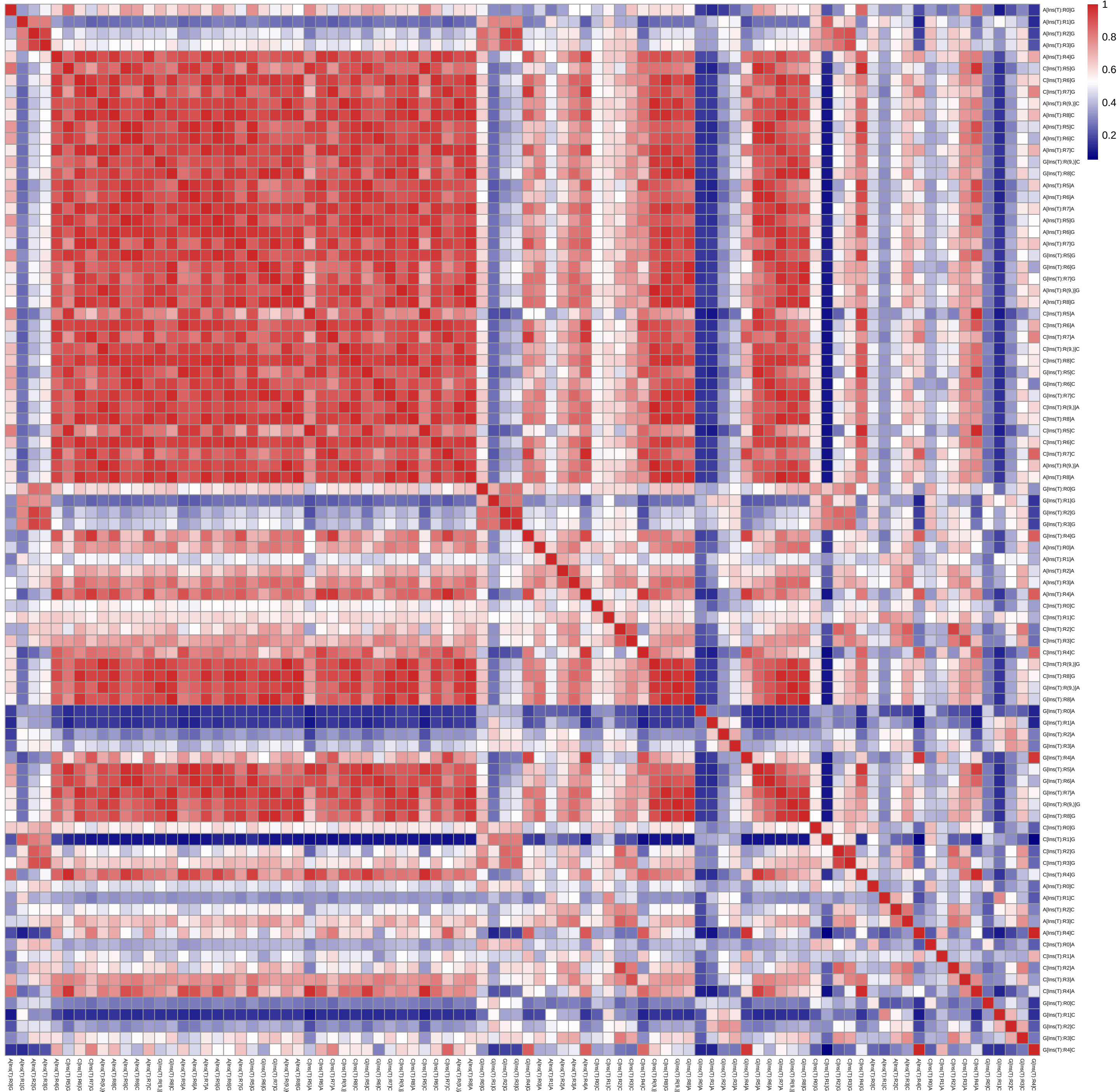
Heatmap (Strict ID89 Order) – Ins_1bp_T
